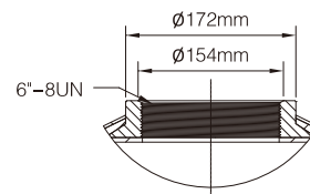
6"—8UN thread Inlet
